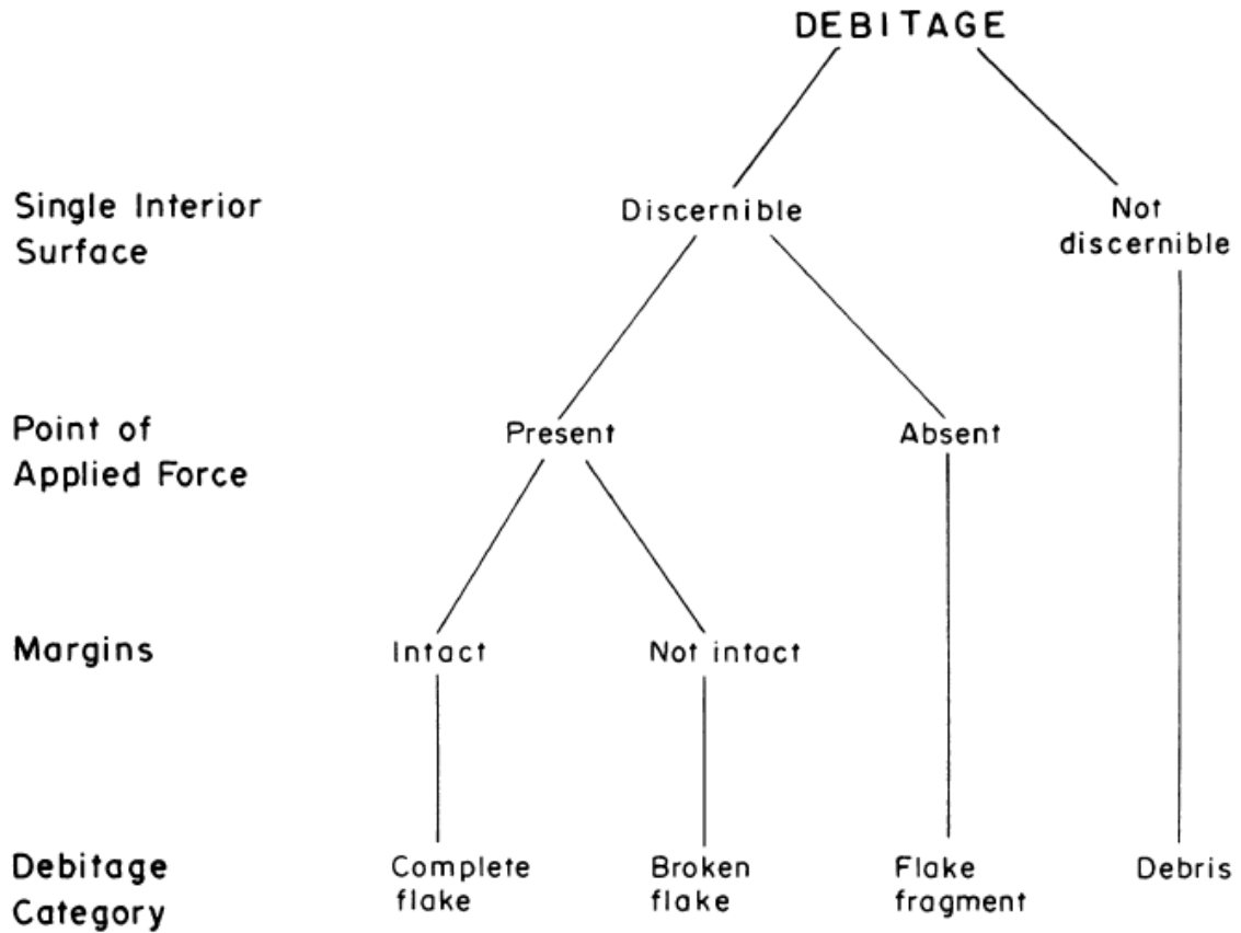
Figure 2. Technological attribute key used to define four debitage categories: complete flakes, broken flakes, flake fragments, and debris.
